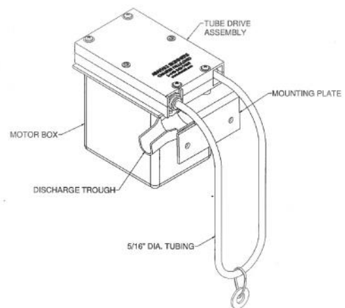
Tube Oil Skimmer STUBE01F
